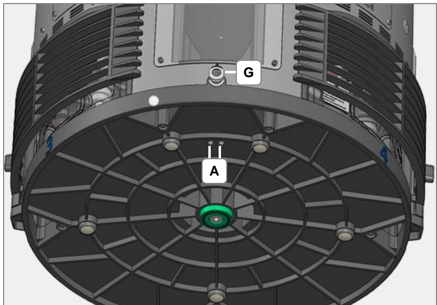
Fig. 11.3.1.1 Bottom view of unit with screw connection
