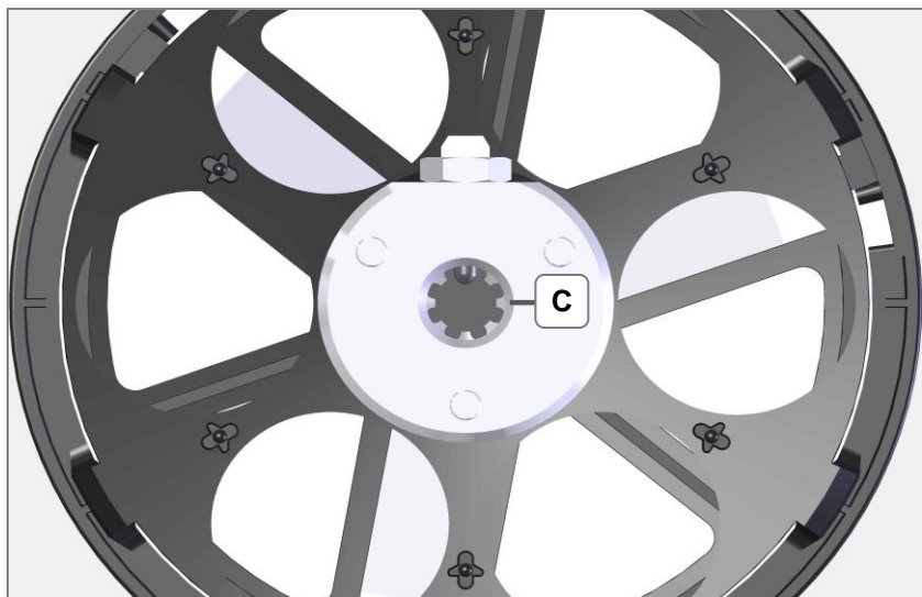
Fig. 9.2.3.3 Basket underside / position of the collar bushing
