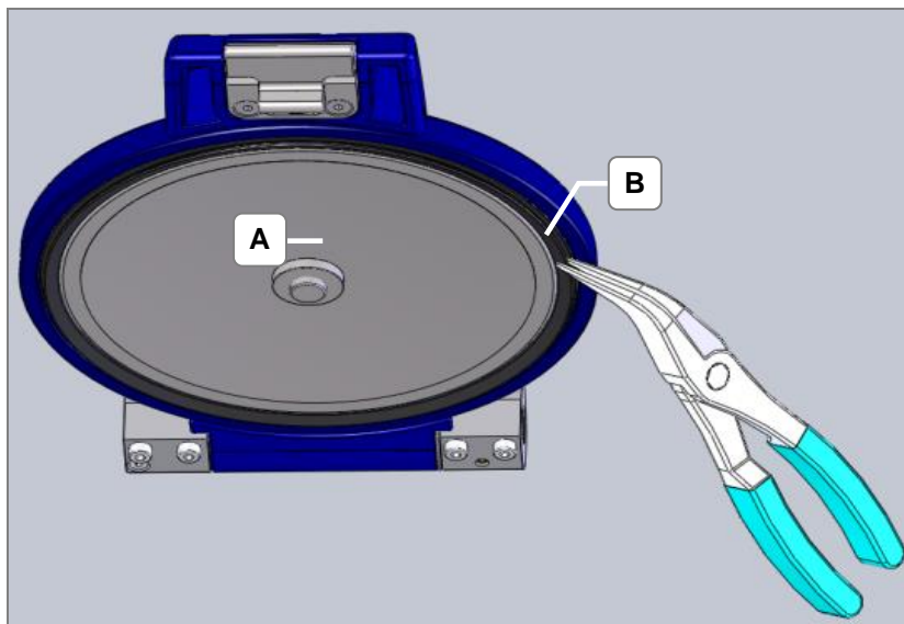
Fig. 10.1.1.1 Removing sealing ring
