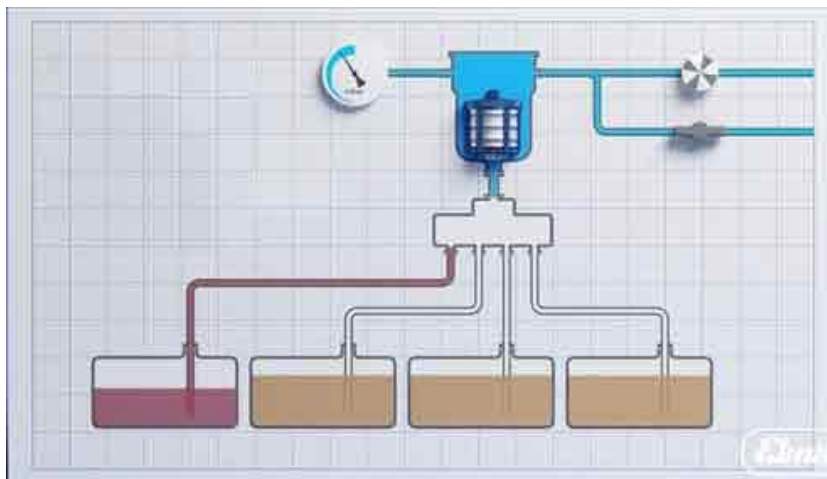
Fig. 3.1.1 Schematic diagram of the functional principle
