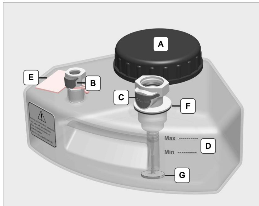
Fig. 3.13.2 Media tanks
