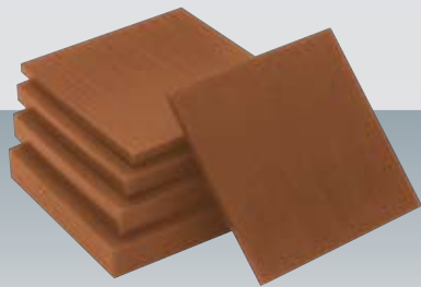
Slice Assortment
