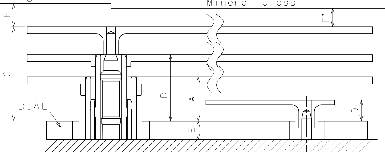
Chronograph minute wheel Chronograph second wheel Small hour hand wheel
